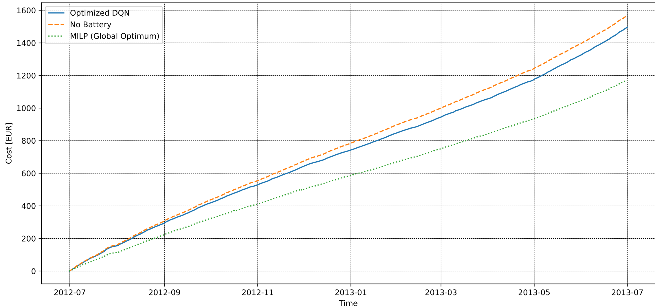
User 113 - Basic Training - Electricity Cost [DQN vs MILP]
